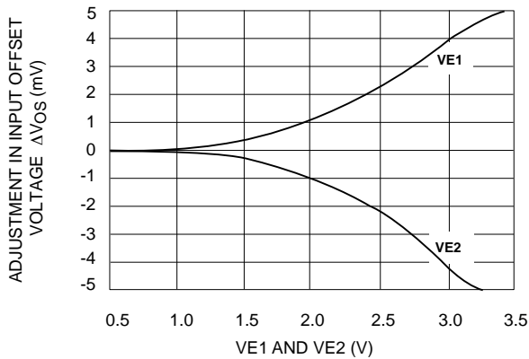
ADJUSTMENT IN INPUT OFFSET VOLTAGE AS A FUNCTION OF VE1 AND VE2
